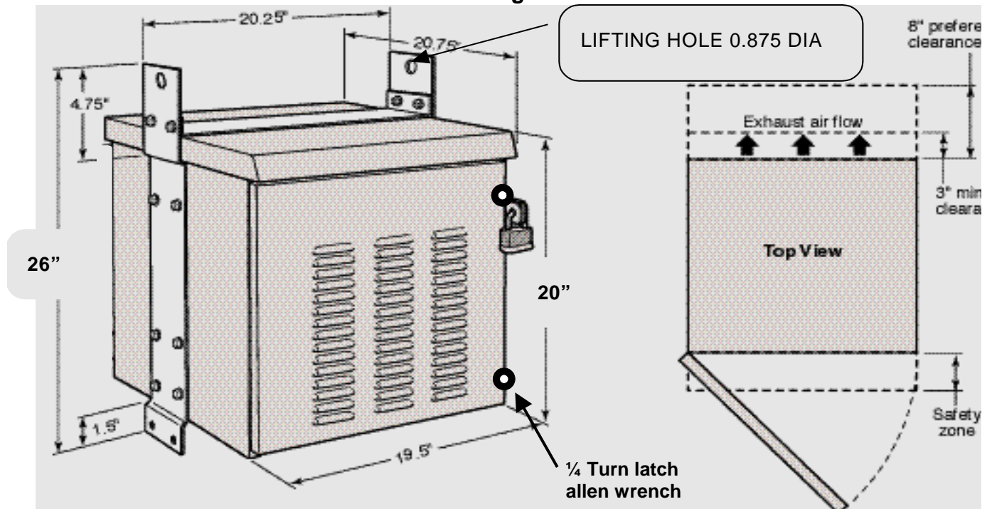
ILLUSTRATION 1-6 OUTLINE DIMENSIONS
